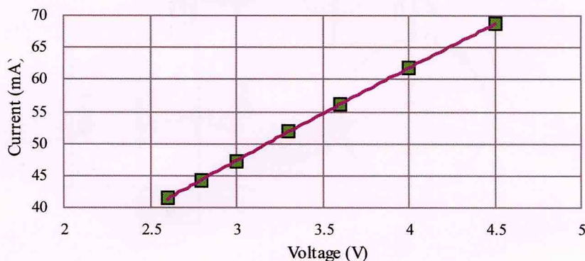
Φ13.2 Vibration Motor (Non-eccentric) V-A Curve
